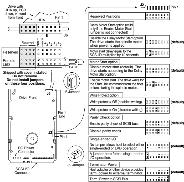
Figure 2. Option select jumpers.
